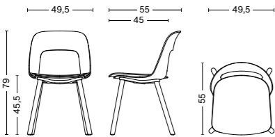
LAYOUT CHAIR 121 Width 49,5 cm Depth 55 cm Height 79 cm Seat height 45,5 cm Weight 6,5 kg
