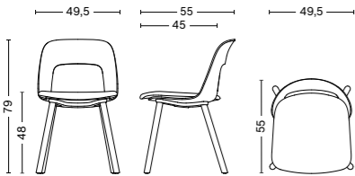
LAYOUT CHAIR 123 Width 49,5 cm Depth 55 cm Height 79 cm Seat height 48 cm Weight 6,8 kg
