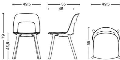
LAYOUT CHAIR 122 Width 49,5 cm Depth 55 cm Height 79 cm Seat height 45,5 cm Weight 6,3 kg
