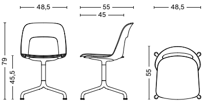
LAYOUT CHAIR 151 Width 50 cm Depth 55 cm Height 79 cm Seat height 45,5 cm Weight 7,9 kg
