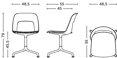
LAYOUT CHAIR 152 Width 50 cm Depth 55 cm Height 79 cm Seat height 45,5 cm Weight 7,7 kg
