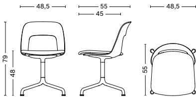
LAYOUT CHAIR 154 Width 50 cm Depth 56 cm Height 80 cm Seat height 48cm Weight 8,6 kg
