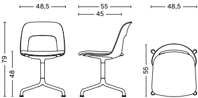
LAYOUT CHAIR 153 Width 50 cm Depth 55 cm Height 79 cm Seat height 48 cm Weight 8,2 kg
