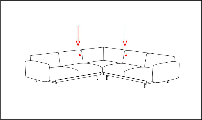
With screw 3, attach the upper linking brackets as shown. Make sure to have both sides facing up .
