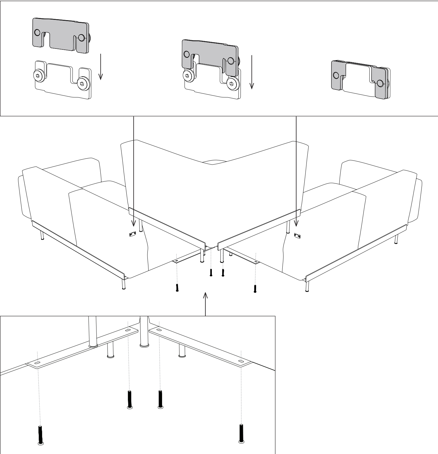
Then, link the upper brackets as shown, and secure the lower linking brackets with the remaining screws underneath.
