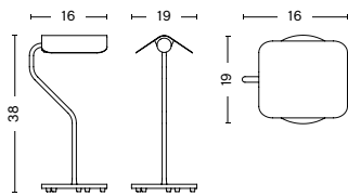
APEX TABLE LAMP Width 19 cm Depth 16 cm Height 38 cm Weight 1,56 kg
