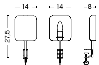
APEX CLIP LAMP Width 14 cm Depth 8 cm Height 27,5 cm Weight 0,57 kg Max. table/shelf thickness 4 cm
